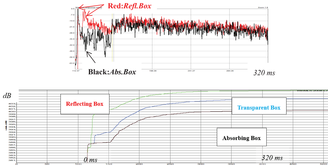
Figure 6 – Upper pane: Impulse response with/without early reflections (Odeon) Lowe pane: Integrated Impulse Response. Red= with early reflections, Black=without early reflections: (Blue= with transparent box, not discussed)
